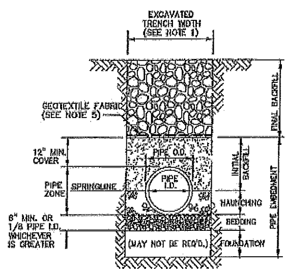
PIPE EMBEDMENT
