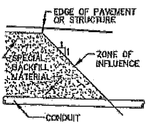
TRANSVERSE ZONE OF INFLUENCE
