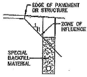
PARALLEL ZONE OF INFLUENCE
